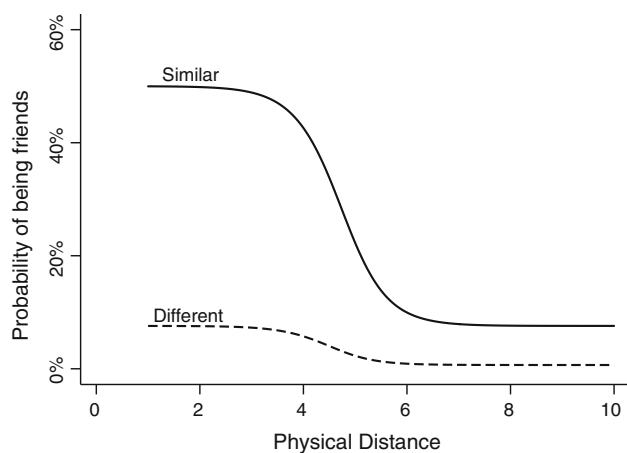
Fig. 2 Friendship selection function when \beta_H = 2.5 , \beta_P = 2.5
